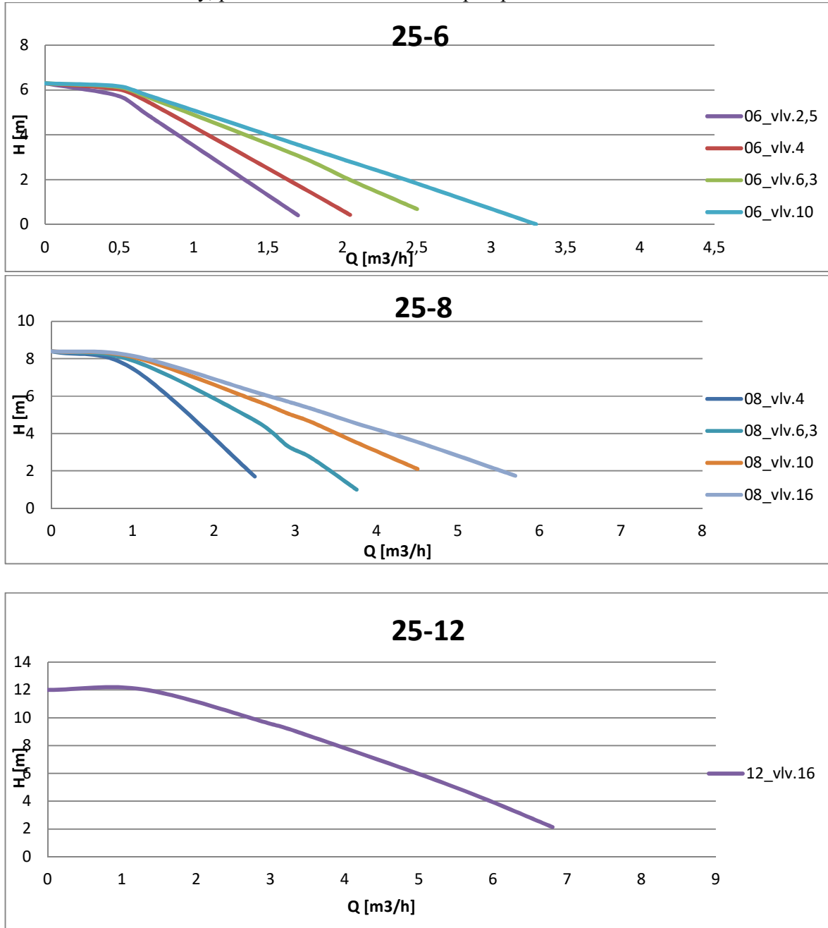
Fig.3. Characteristics of water pump groups
