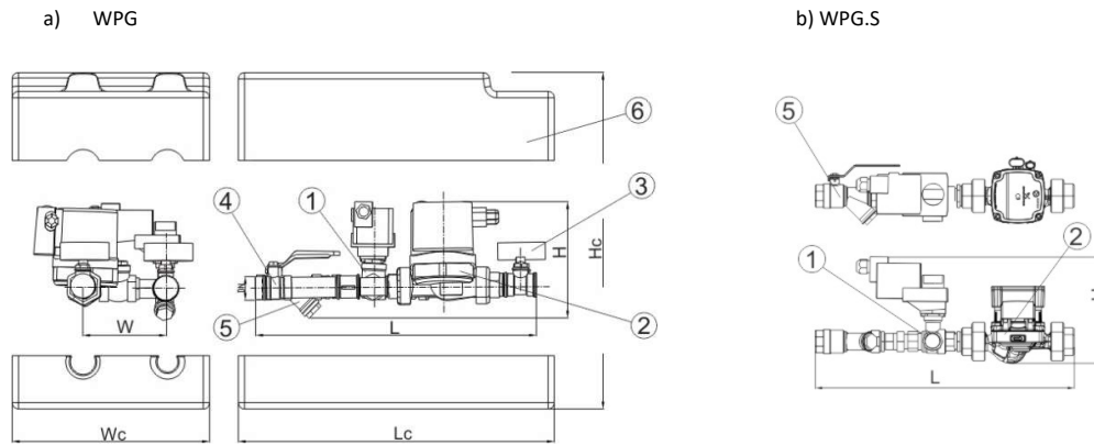
Fig.1. Structure of water pump group
